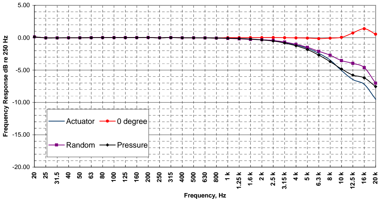
Microphone Frequency Response Type 4189 S/N 2048567 : Measured 30 Apr 2012
